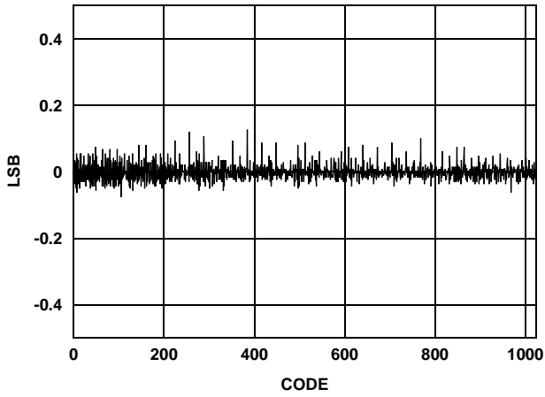
FIGURE 36. DIFFERENTIAL NONLINEARITY
